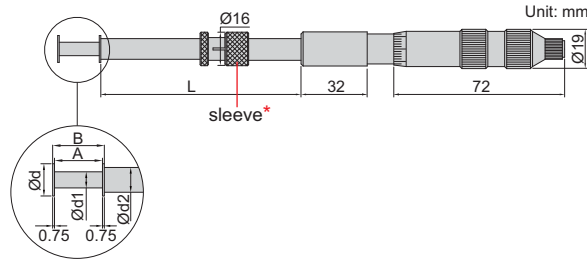
measure width of keyway
